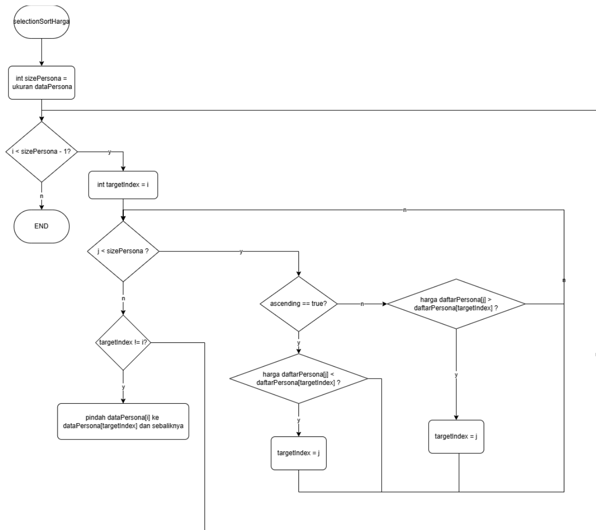
gambar 1.13 selection sort ascending dan descending
