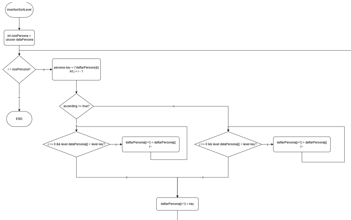
gambar 1.12 insertion sort ascending dan descending
