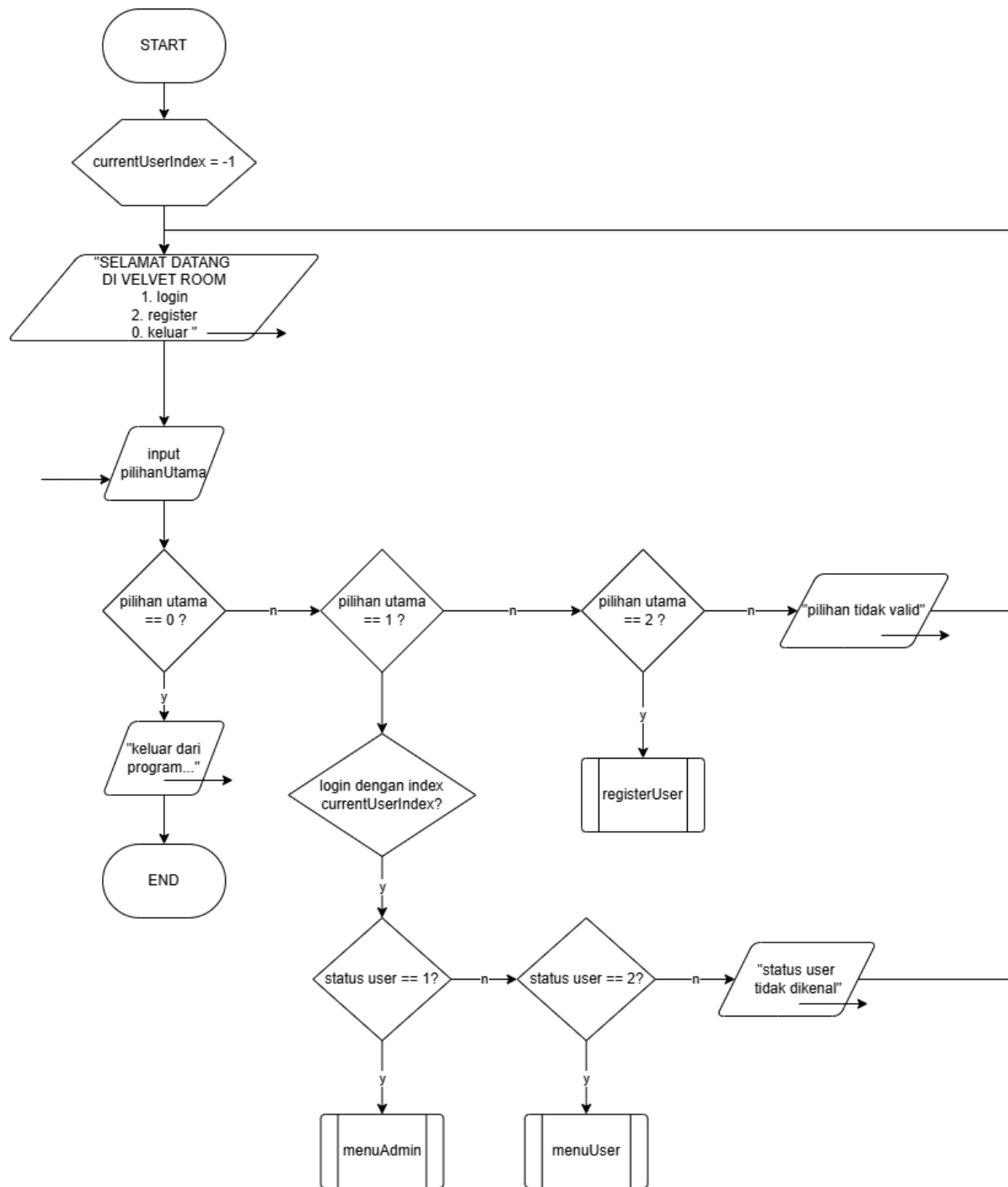
gambar 1.1 main program
